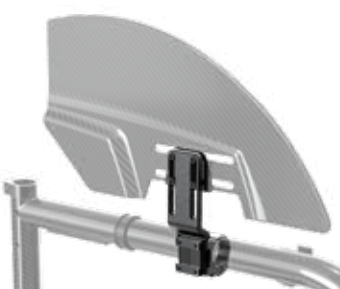
SG ↑ Plastic fender side guards offset bracket (removable)
