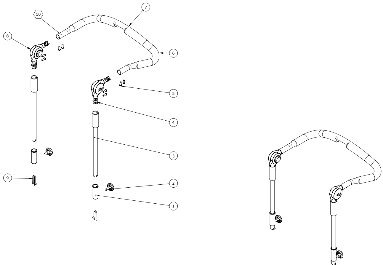
Item numbers Height adjustable kit for angle adjustable push brace (95630-10)
