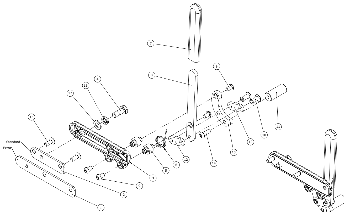
Item numbers for Left side rear wheel handbrake
