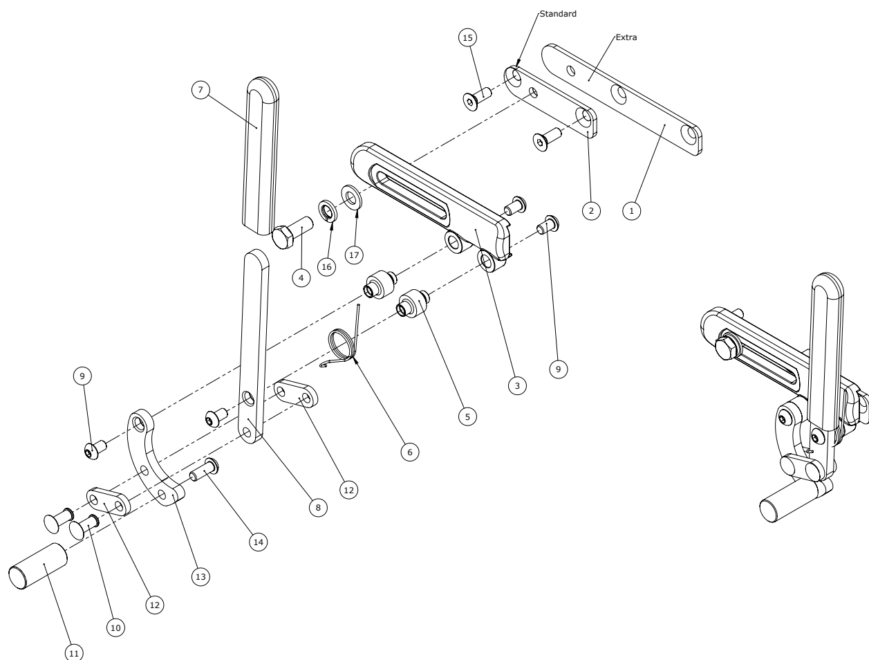
Item numbers for Right side rear wheel handbrake 20" 22" 24"
